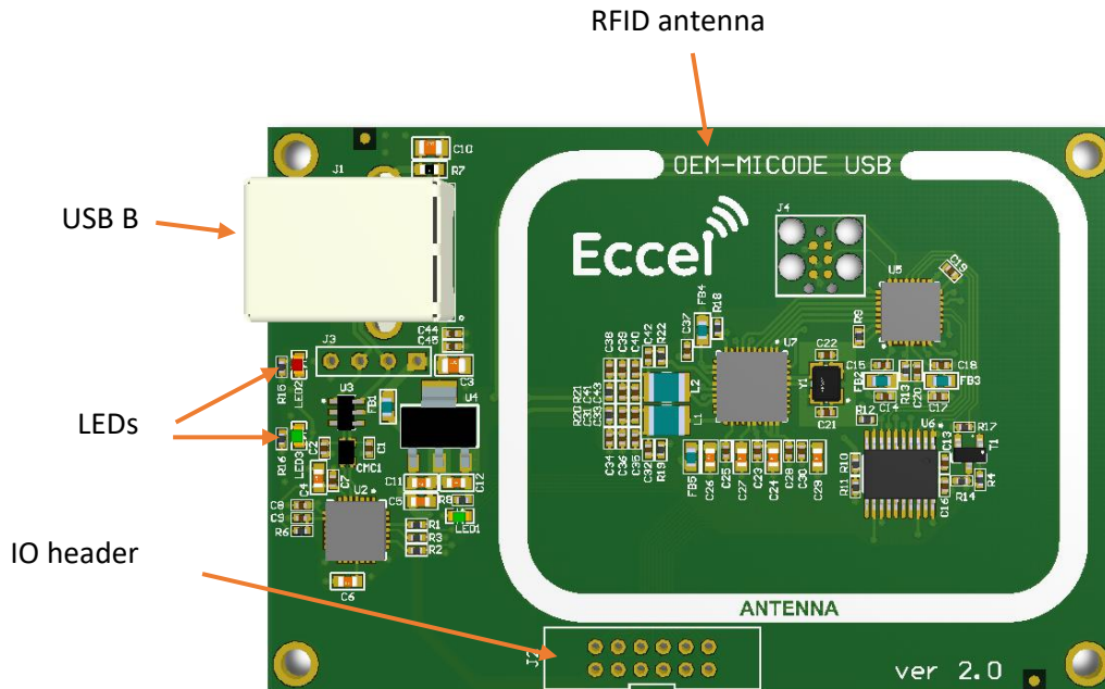
Figure 1. OEM MICODE USB TURBO version
