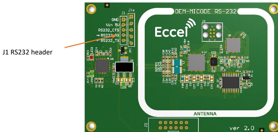
Figure 2. OEM MICODE RS232 TURBO version
