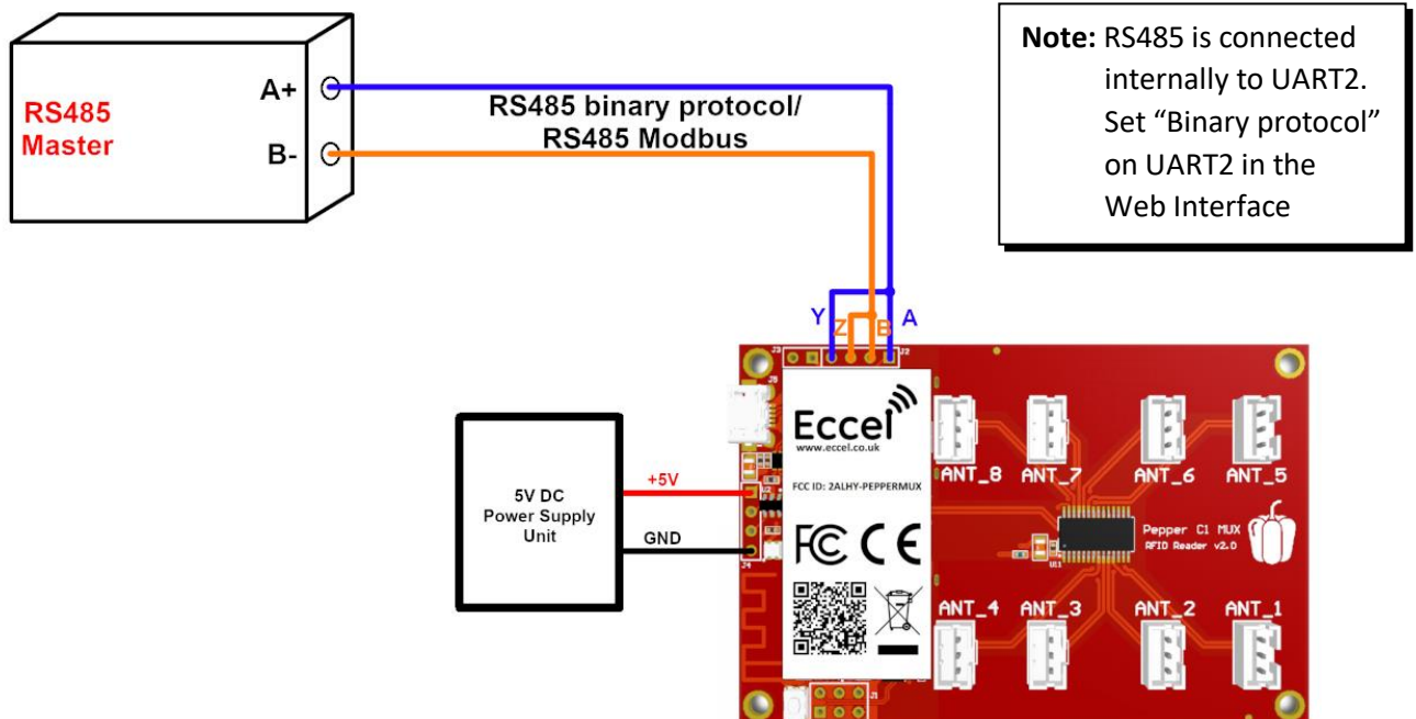
Figure 3-7. Pepper C1 FCC MUX RS485 - half duplex connection schematic
