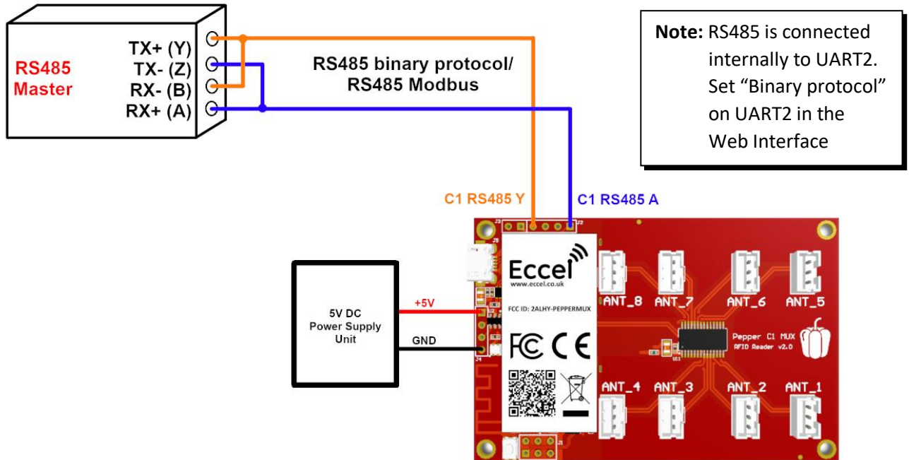
Figure 3-6. Pepper C1 FCC MUX RS485 - half duplex connection schematic
