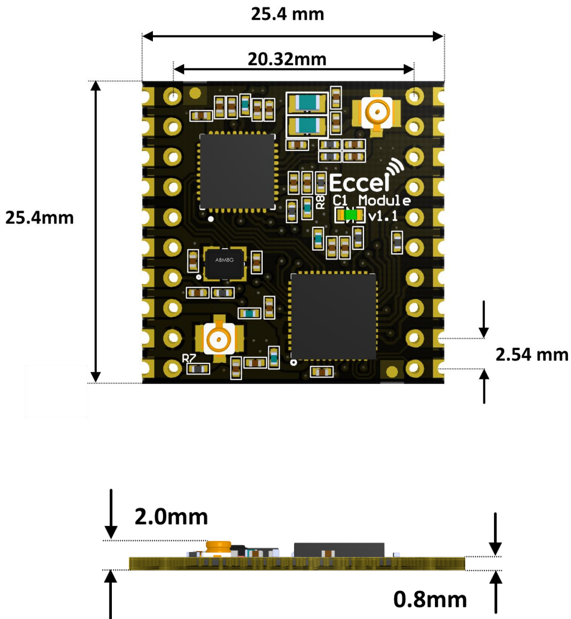
Figure 4-1 Pepper C1 module dimension
